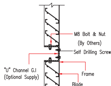
Horizontal Joint Details
