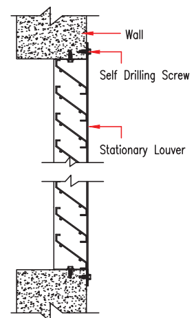
Wall Installation
