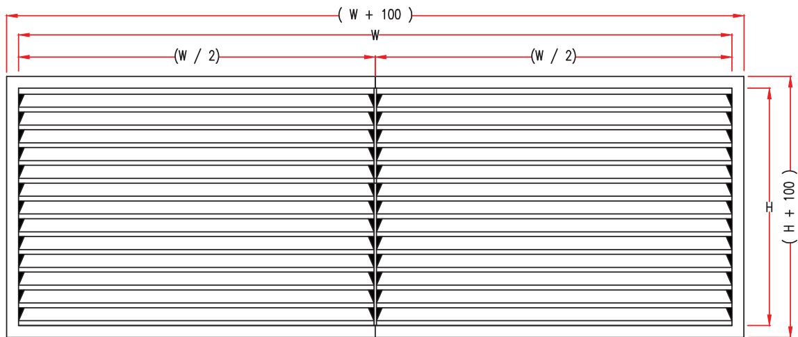
Multiple Section Front View
