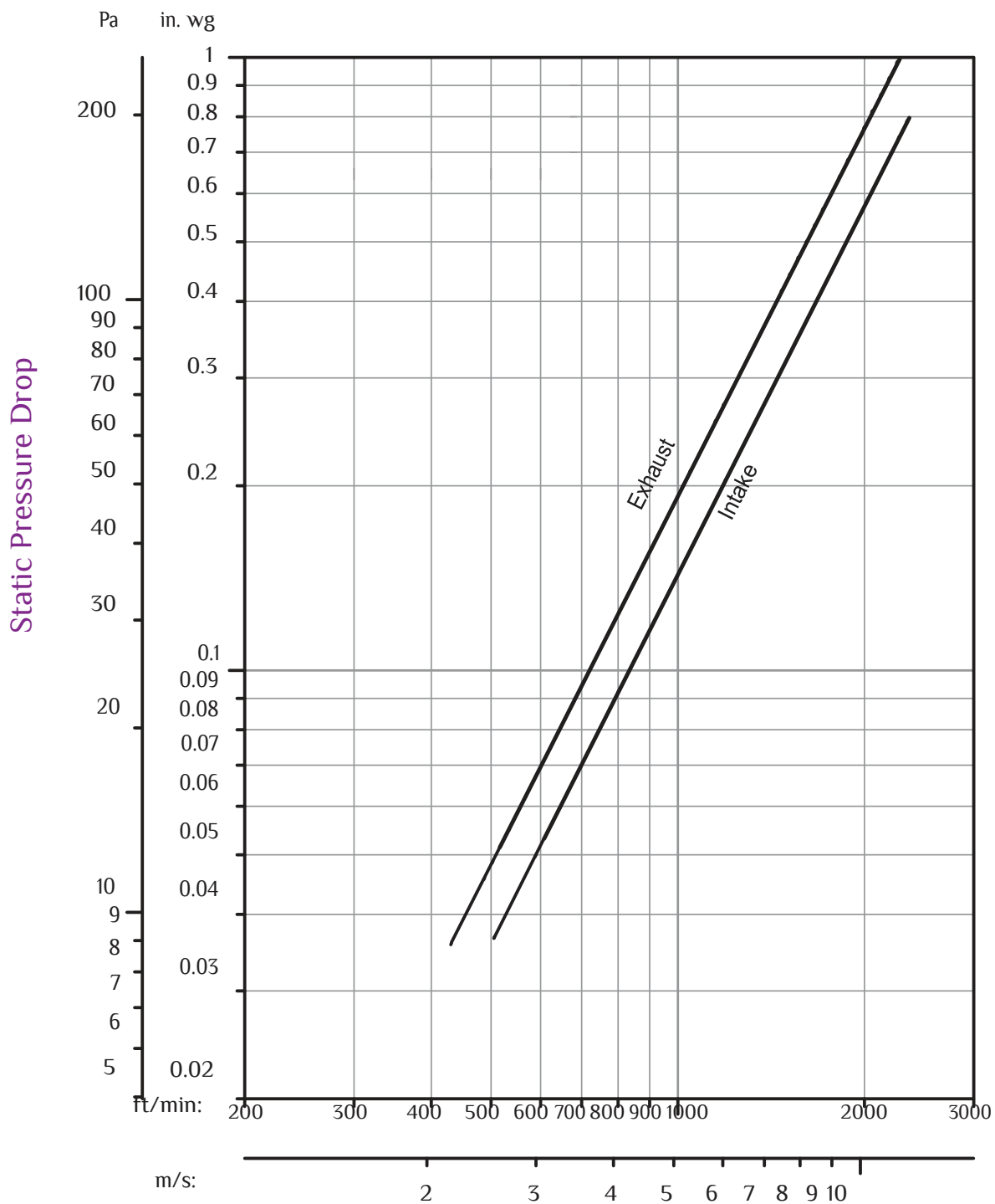
Free Area Velocity & Pressure Drop
